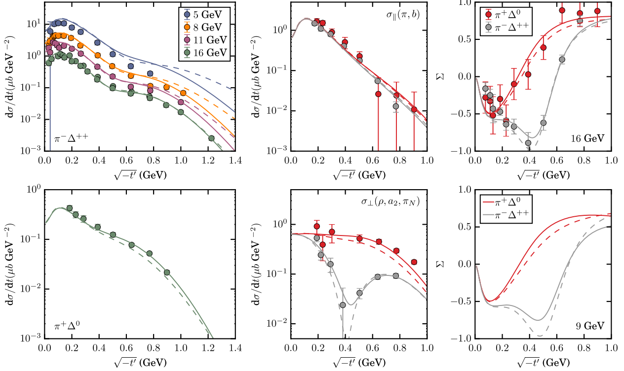
Fig. 2. The comparison of pole (dashed) and cut (solid) models with the available (unpolarized) differential cross section and beam asymmetry data from Refs. [28,27,41]. In the bottom right panel, we show the predictions for E_{\text{lab}} = 9 GeV which is relevant for the GlueX experiment. The data and model for \gamma p \rightarrow \pi^+ \Delta^0 have been rescaled by a factor of 3 to compensate the overall isospin coefficient in Eq. (5).
