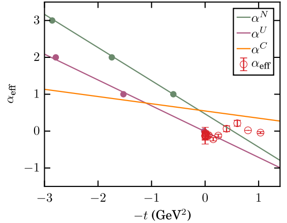
Fig. 1. The t dependence of some selected trajectories. The effective trajectory of the cross section \alpha_{\text{eff}}(t) (red) is extracted with the aid of a fit to the data with the function in Eq. (10). The green and purple solid curves illustrate the Regge trajectories used in this work (see text), together with observed particles. The orange line depicts the \rho \otimes \mathbb{P} or a_2 \otimes \mathbb{P} cut trajectory. (For interpretation of the references to color in this figure legend, the reader is referred to the web version of this article.)
